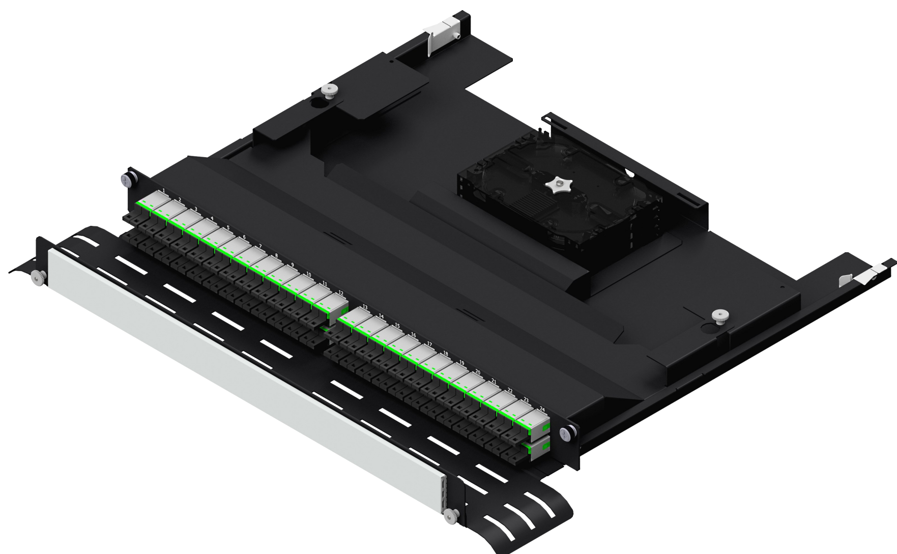
Layout front panel 48xLSH(E2000)-Duplex
