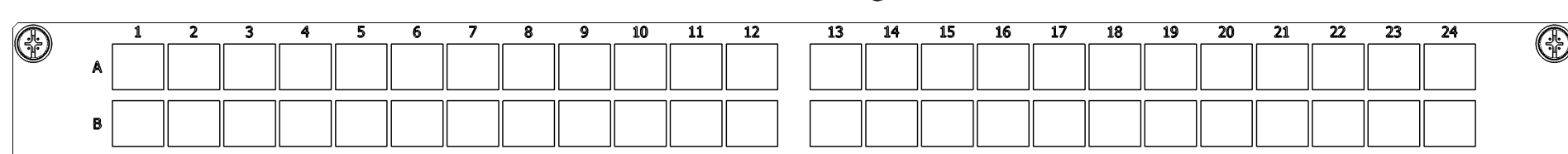
Layout front panel 48xLSH(E2000)-Duplex
